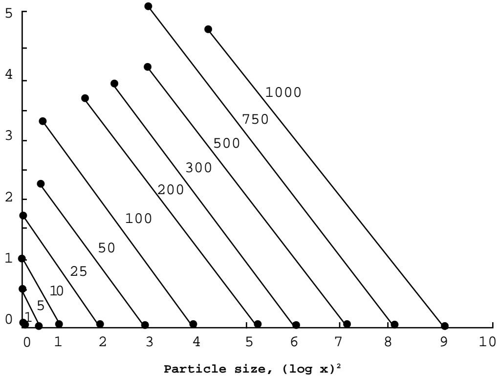
Figure 1. Product cleanliness levels
